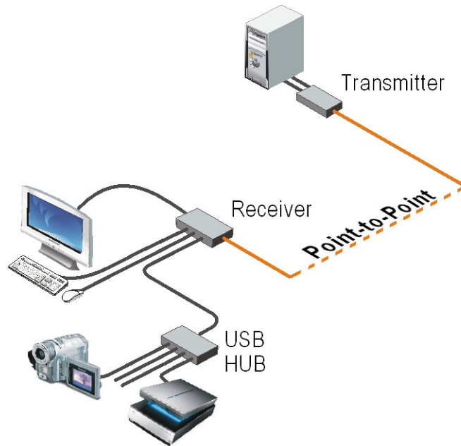
Figure 5. CrystalView EX HDMI Installation
